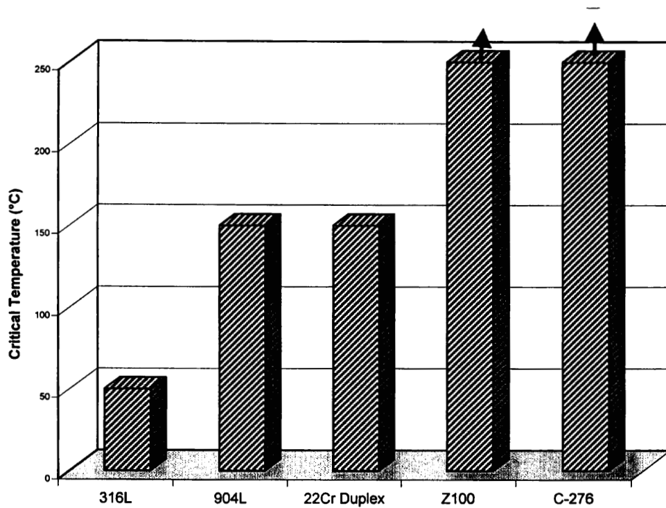
Figure 2. Temperature for the onset of chloride SCC in 3% sodium chloride solution.
