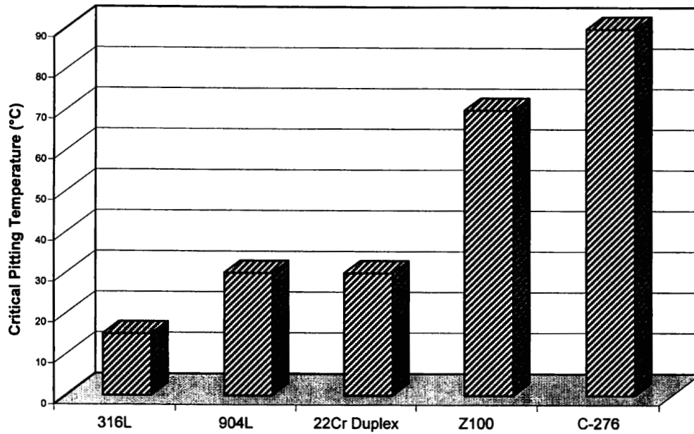
Figure 1. Critical pitting temperature in 10% ferric chloride (ASTM G48A).
