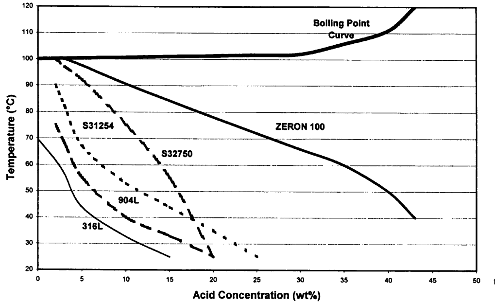
Figure 4. Iso-corrosion curves (0.1 mm/y) for some stainless steels in sulphuric acid plus 2,000 mg/l chloride.
