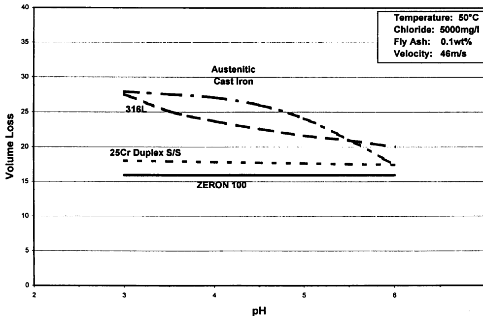
Figure 6. Comparative erosion corrosion data for some FGD slurry pump alloys.
