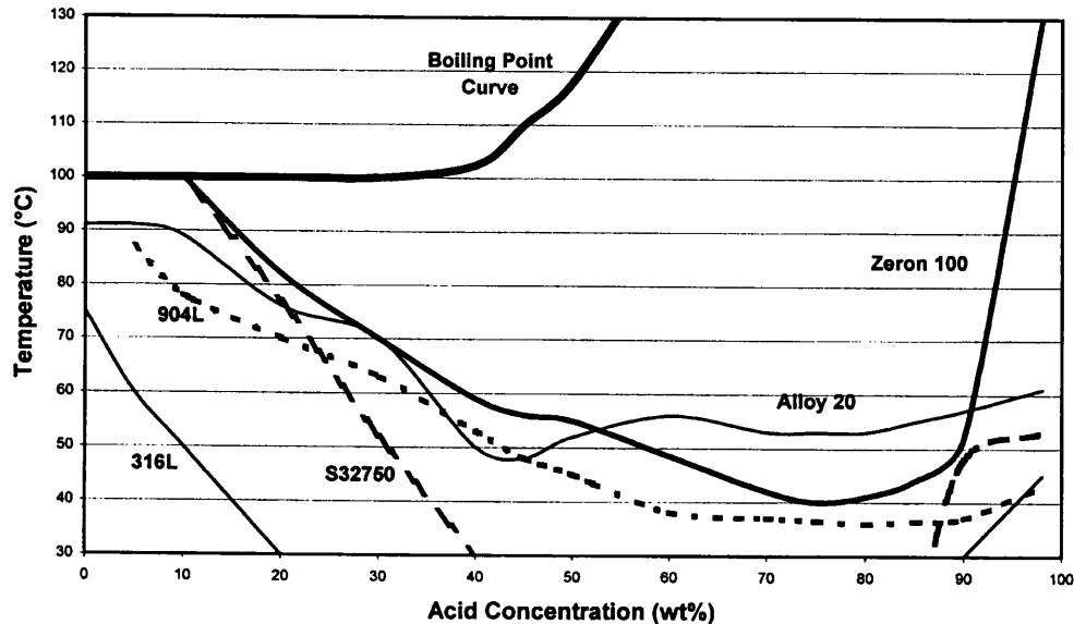
Figure 3. Iso-corrosion curves (0.1 mm/y) for some stainless steels in sulphuric acid.
