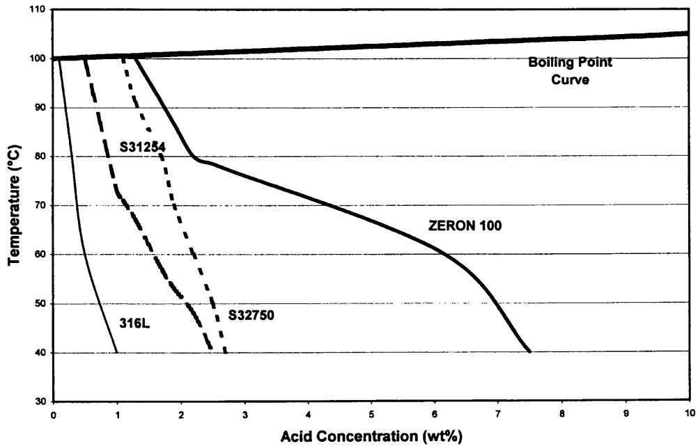
Figure 5. Iso-corrosion curves (0.1 mm/y) for some stainless steels in hydrochloric acid.
